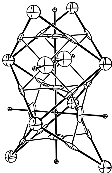
BODY-CENTERED CUBIC
