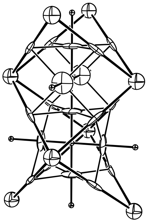
BODY-CENTERED CUBIC
