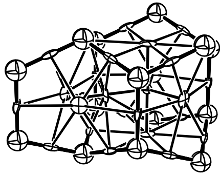
HEXAGONAL DIAMOND
