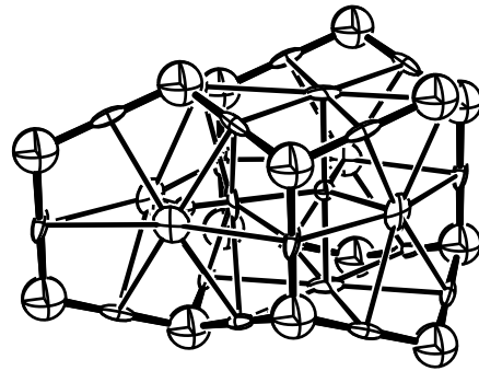
HEXAGONAL DIAMOND
