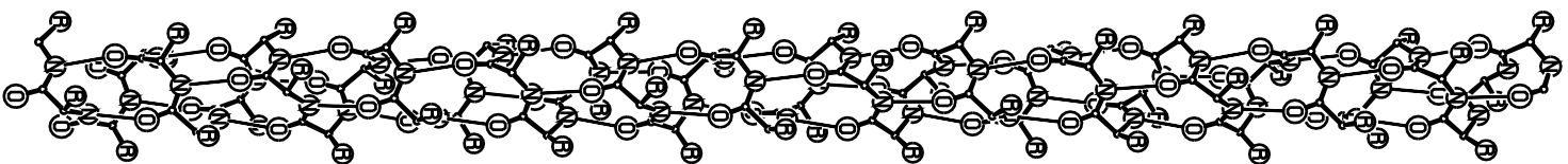
47/13 ALPHA HELIX
