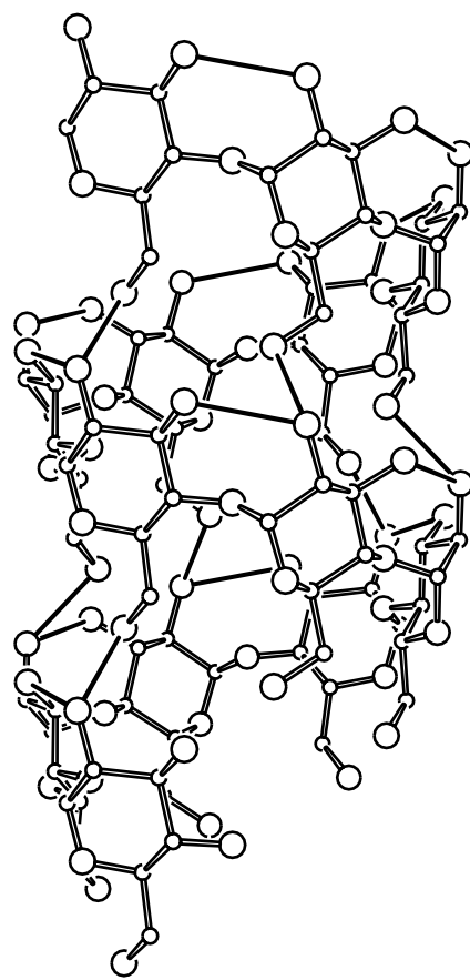
PROPOSED MODEL FOR \gamma -AMYLOSE
