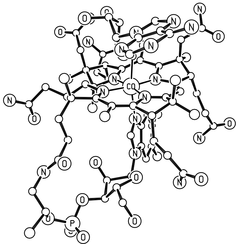
5,6-DIMETHYLBENZIMIDAZOLYL-COBAMIDE COENZYME
