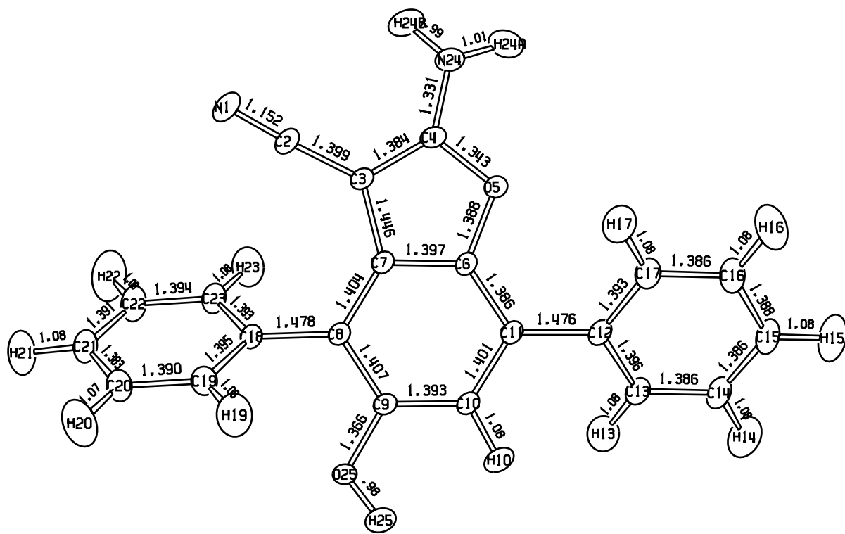
2-AMINO-3-CYANO-4,7-DIPHENYL-5-HYDROXY-BENZOFURAN
