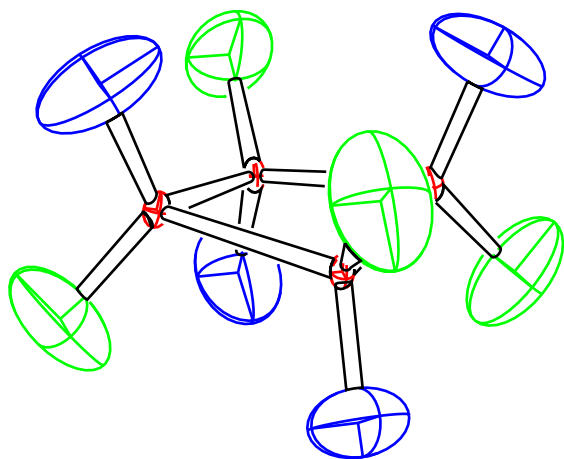
CYCLOBUTANE
