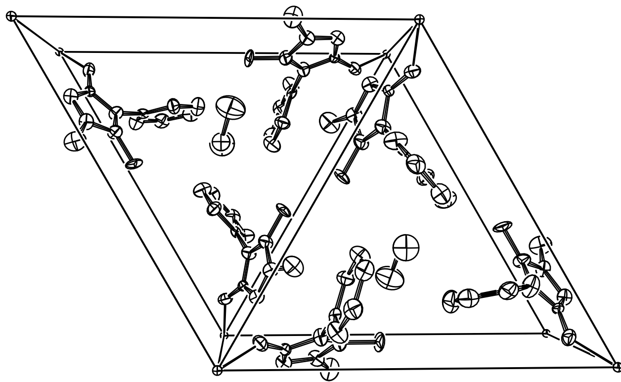
MAGNESIUM HEXANTIPYRINE PERCHLORATE
