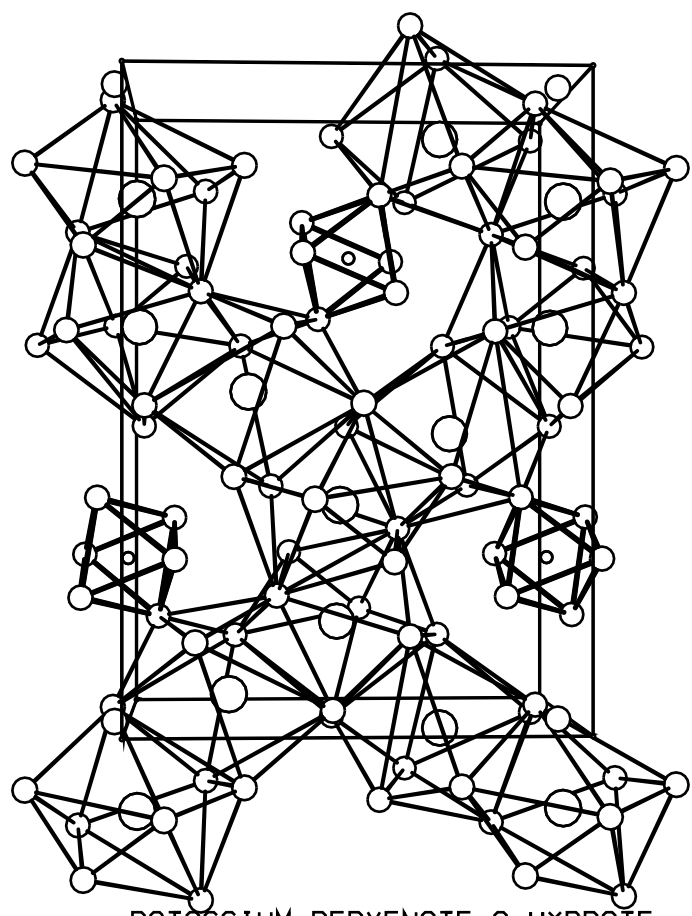
POTASSIUM PERXENATE 9-HYDRATE
